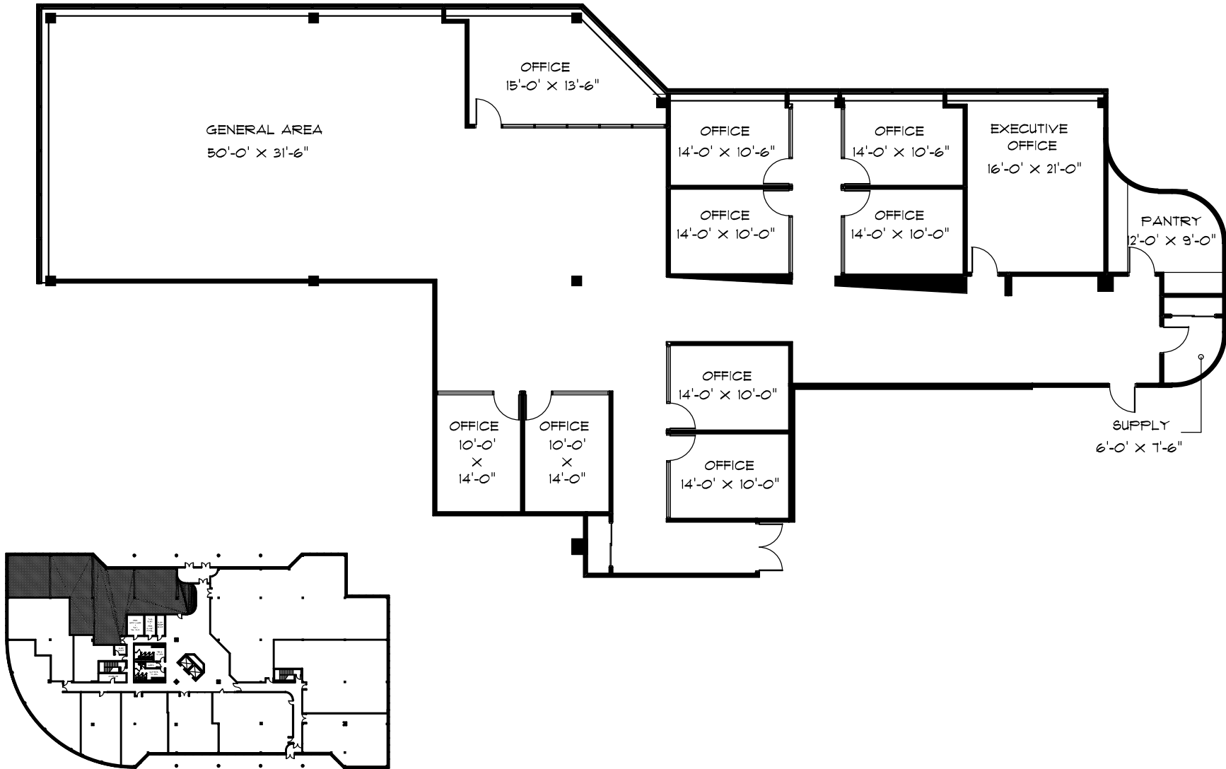
KEY PLAN
